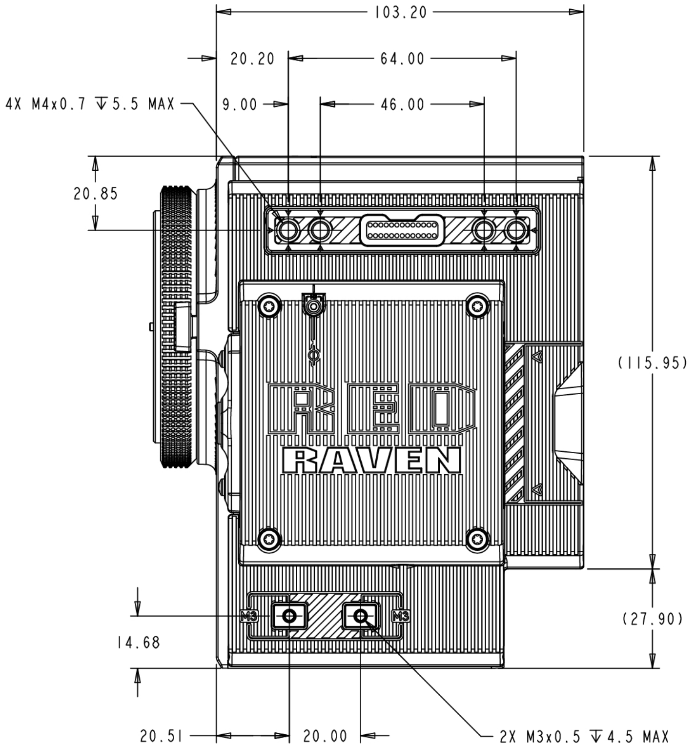
图：RAVEN Side View (Right)
