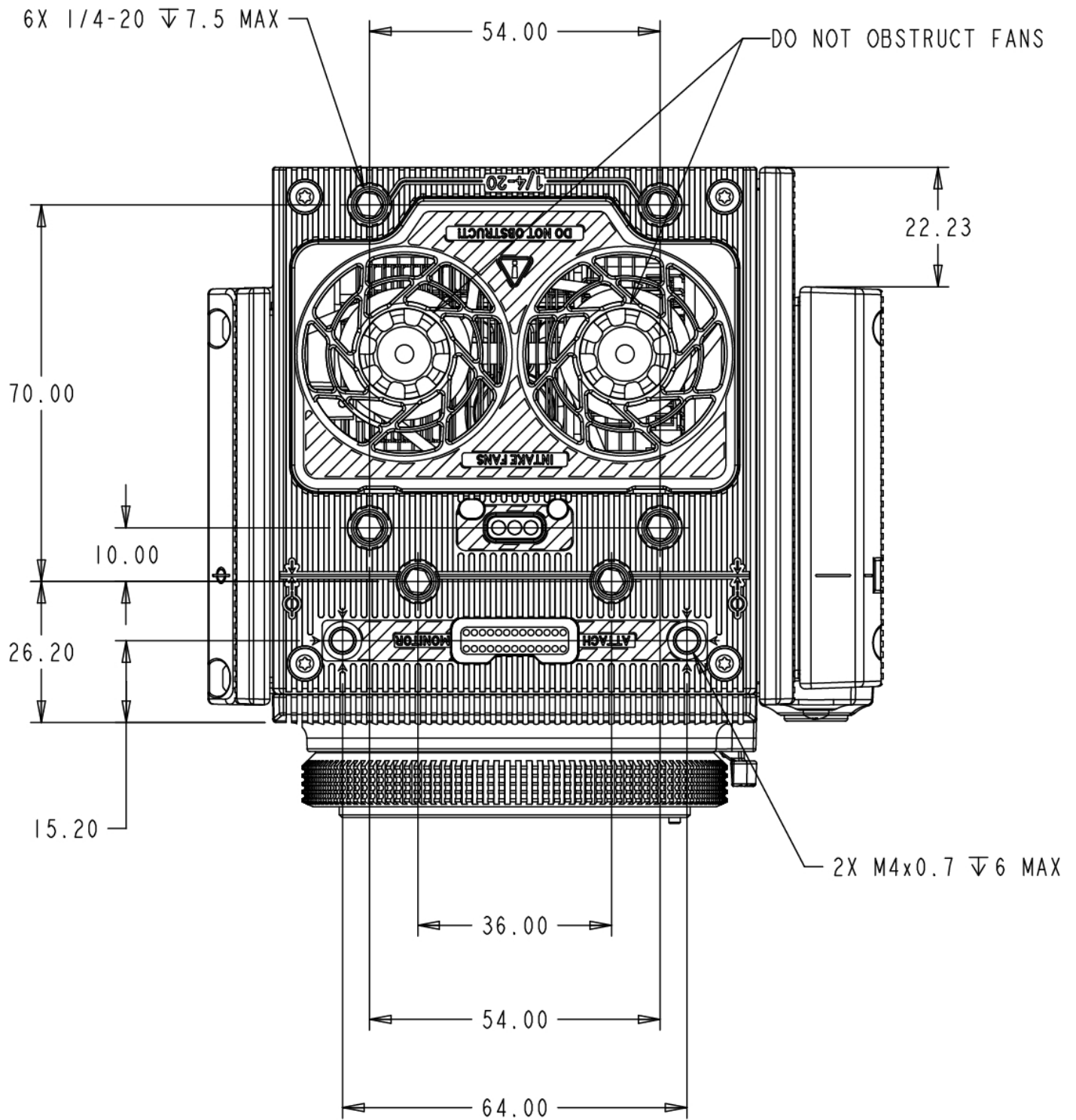
图：RAVEN Top View
